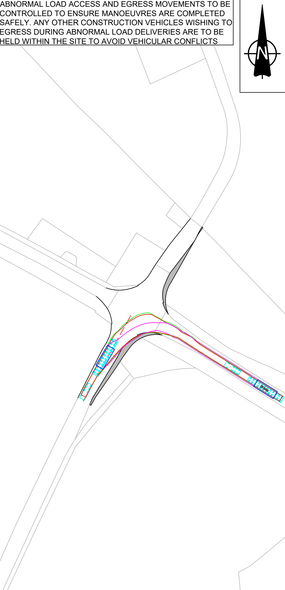
INSET D: 31m 132kV TRANSFORMER VEHICLE WESTBOUND LEFT TURN INTO ACCESS - SCALE 1:1000
