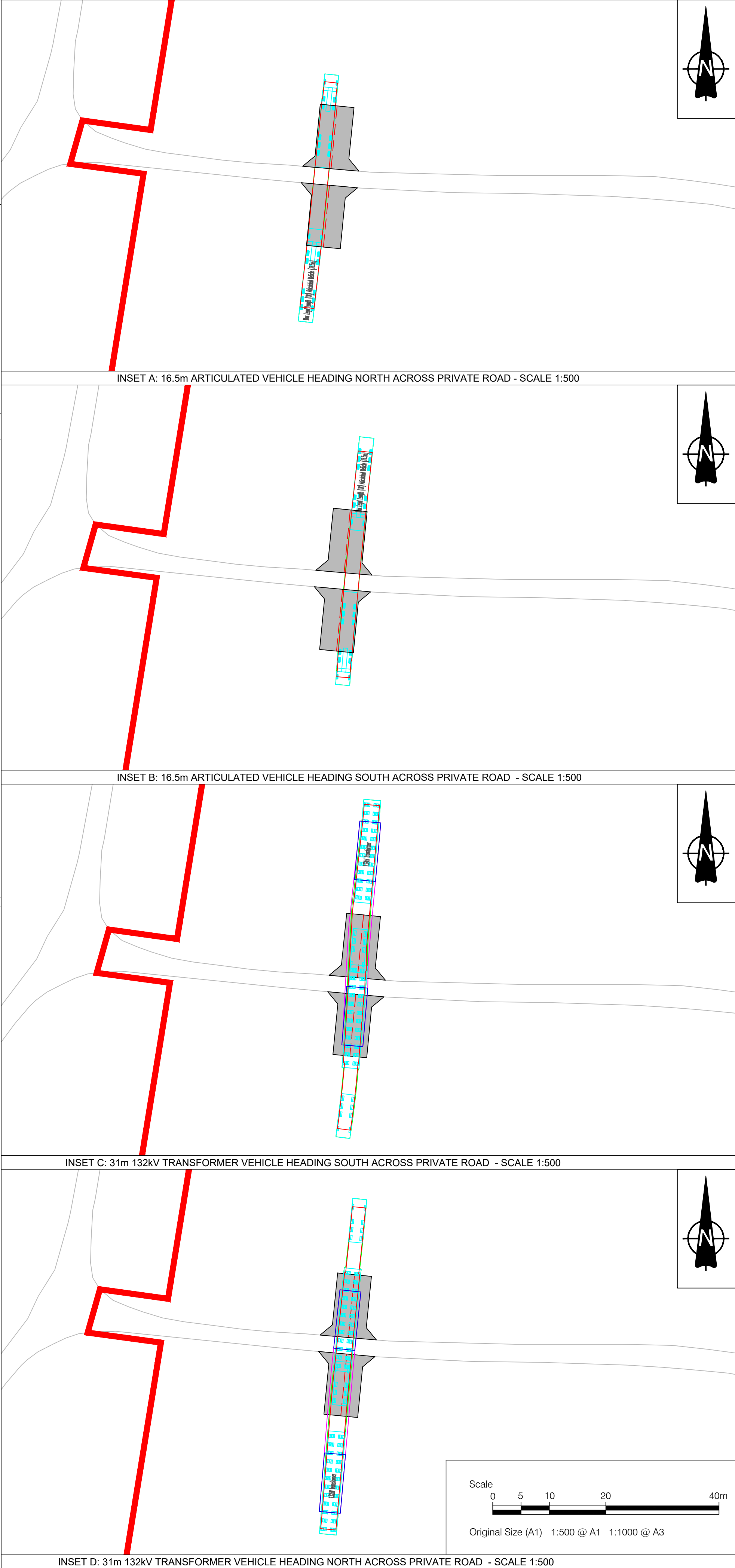
INSET D: 31m 132kV TRANSFORMER VEHICLE HEADING NORTH ACROSS PRIVATE ROAD - SCALE 1:500
