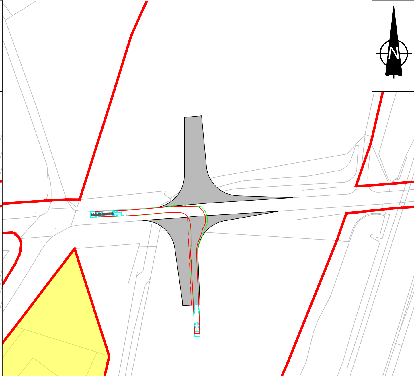
INSET D: 16.5m ARTICULATED VEHICLE HEADING EAST ON COMMON LANE AND TURNING RIGHT INTO ACCESS - SCALE 1:1000
