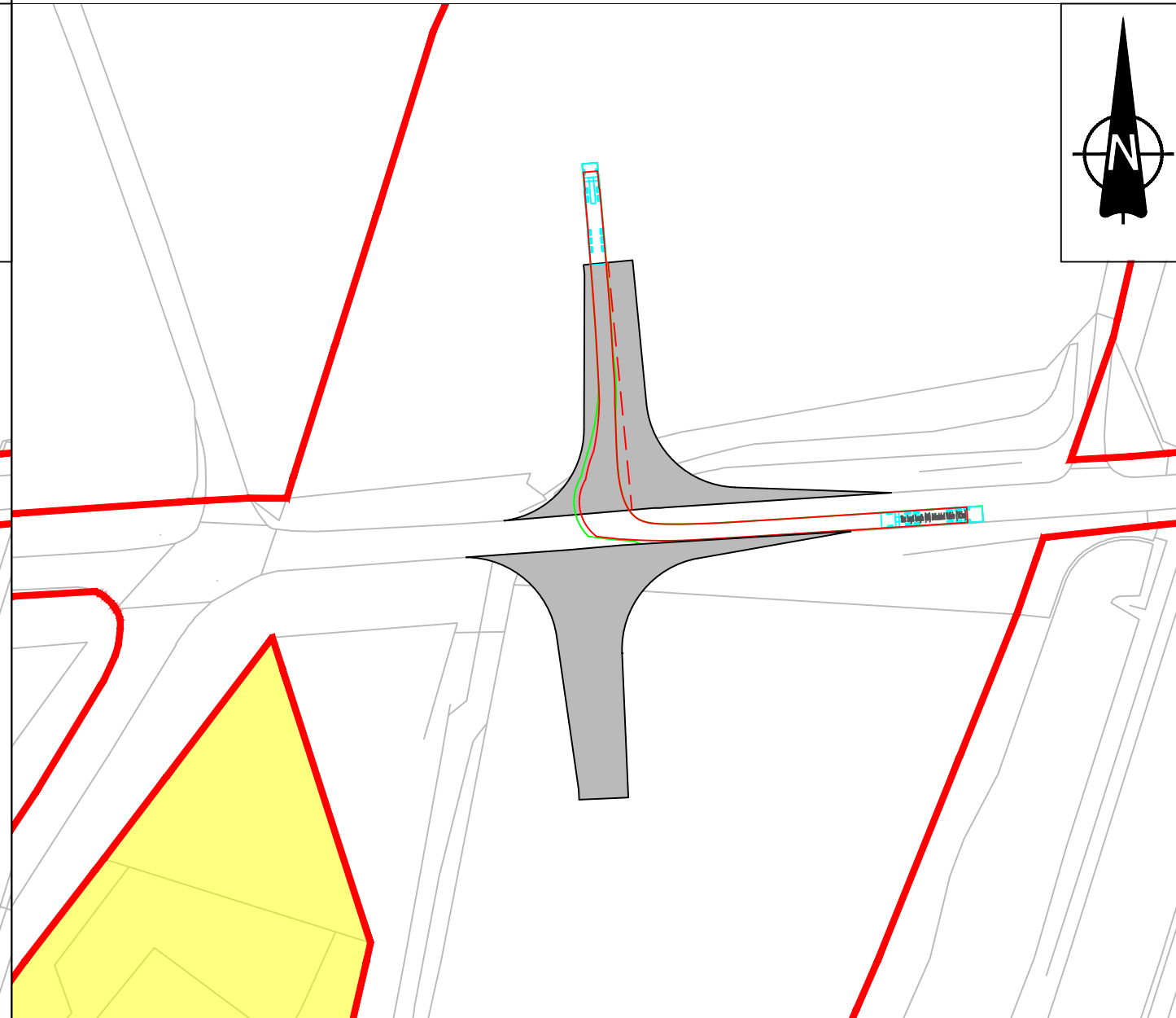
INSET F: 16.5m ARTICULATED VEHICLE HEADING WEST ON COMMON LANE AND TURNING RIGHT INTO ACCESS - SCALE 1:1000
