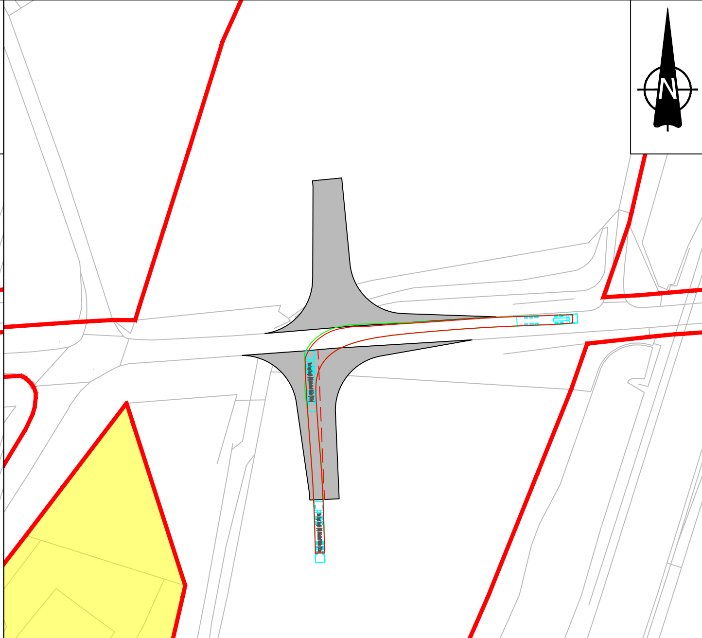
INSET B: 16.5m ARTICULATED VEHICLE TURNING RIGHT OUT OF ACCESS ONTO COMMON LANE HEADING EAST - SCALE 1:1000
