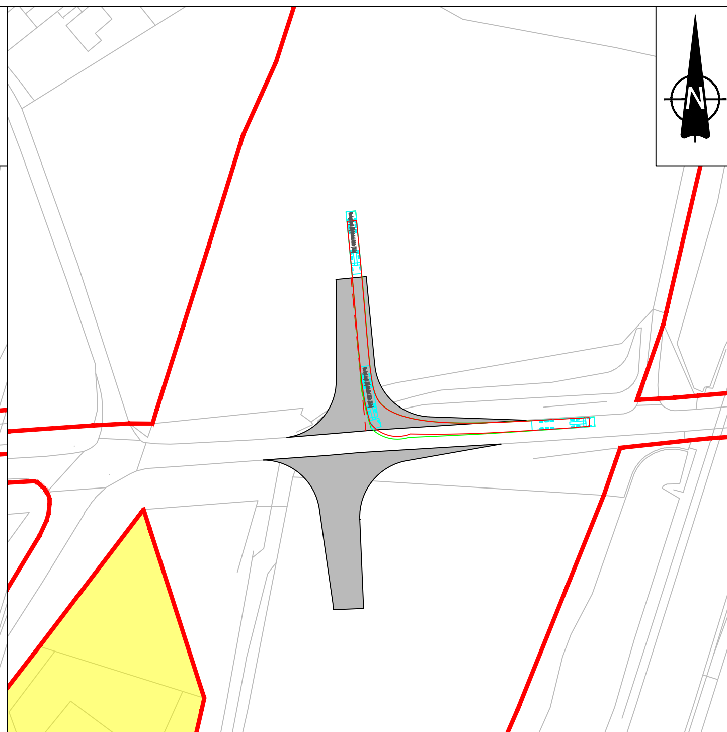
INSET B: 16.5m ARTICULATED VEHICLE TURNING LEFT OUT OF ACCESS ONTO COMMON LANE HEADING EAST - SCALE 1:1000
