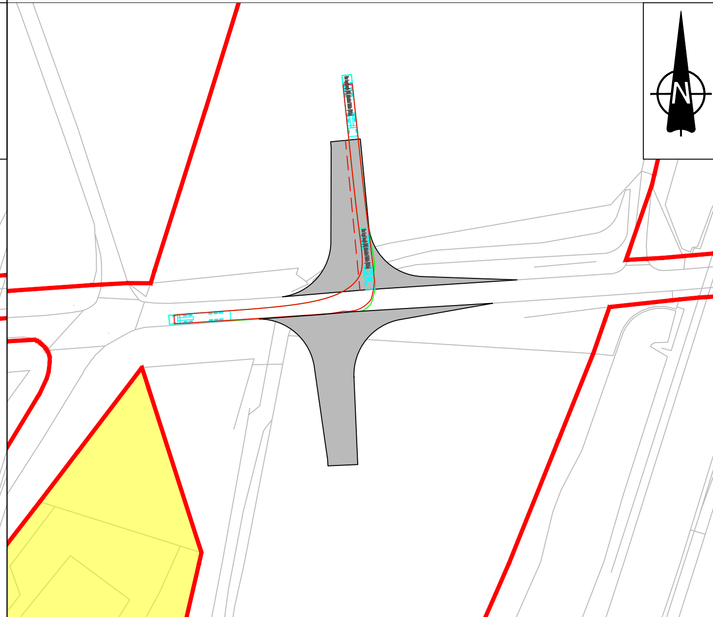
INSET D: 16.5m ARTICULATED VEHICLE TURNING RIGHT OUT OF ACCESS ONTO COMMON LANE HEADING WEST - SCALE 1:1000
