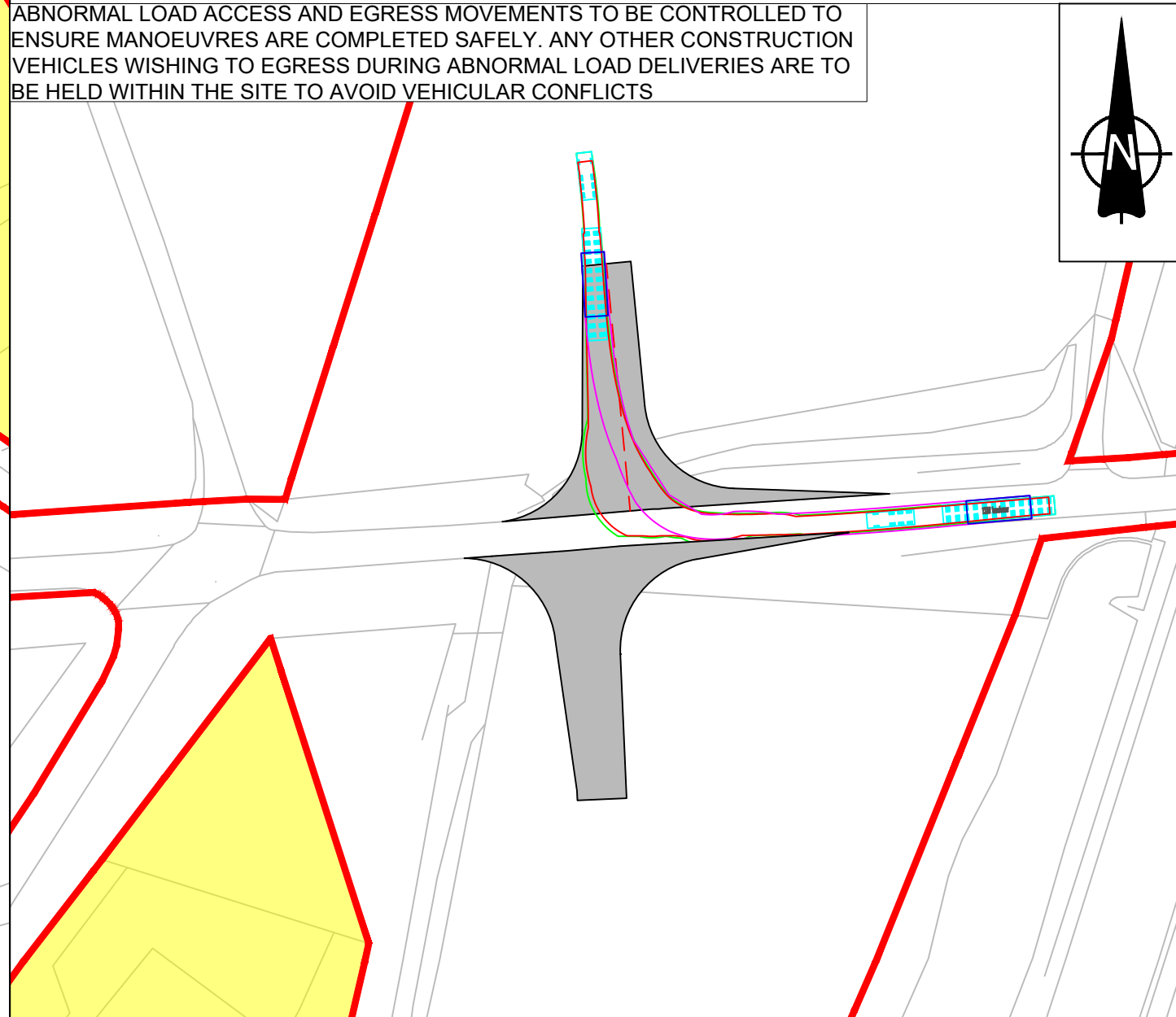
INSET E: 31m 132kV TRANSFORMER VEHICLE HEADING WEST ON COMMON LANE AND TURNING RIGHT INTO ACCESS - SCALE 1:1000
