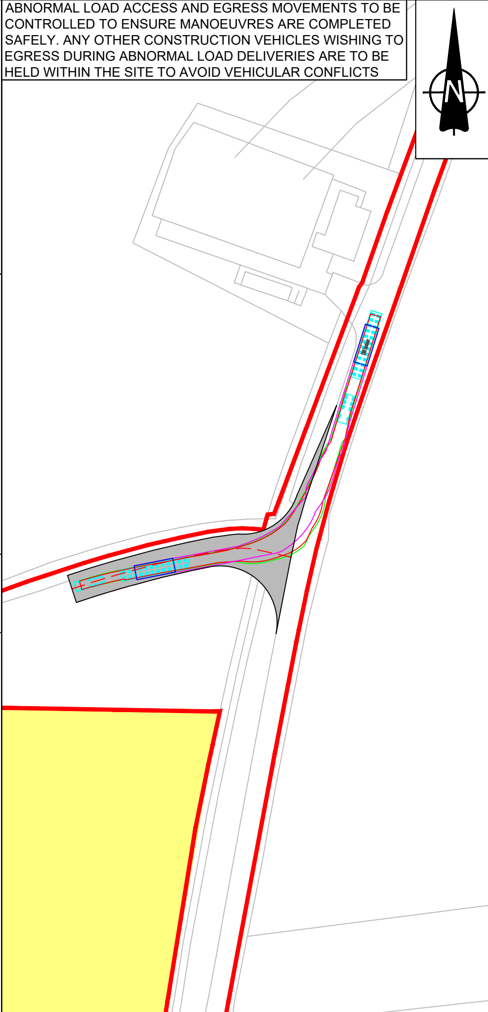
INSET A: 31m 132kV TRANSFORMER VEHICLE SOUTHBOUND RIGHT TURN INTO ACCESS - SCALE 1:1000
