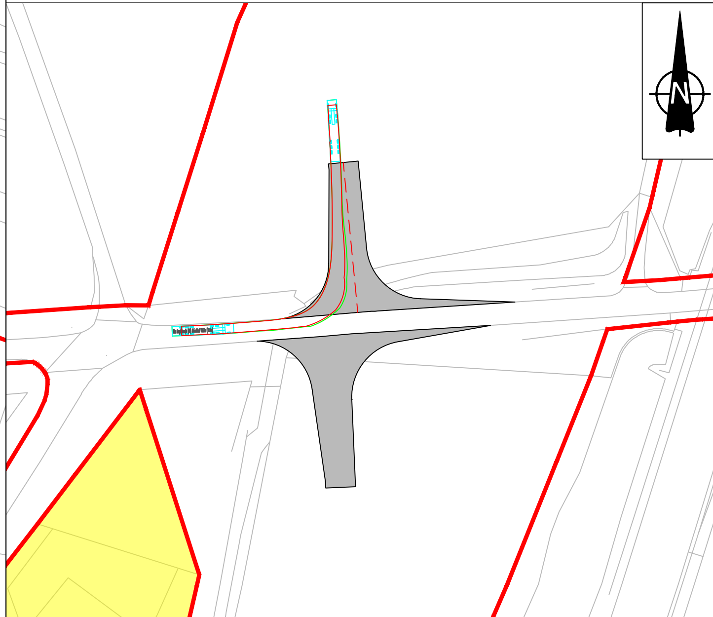
INSET C: 16.5m ARTICULATED VEHICLE HEADING EAST ON COMMON LANE AND TURNING LEFT INTO ACCESS - SCALE 1:1000
