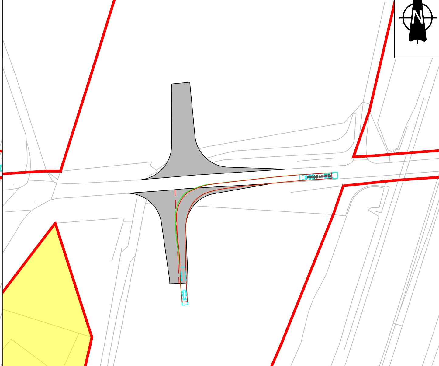
INSET F: 16.5m ARTICULATED VEHICLE HEADING WEST ON COMMON LANE AND TURNING LEFT INTO ACCESS - SCALE 1:1000
