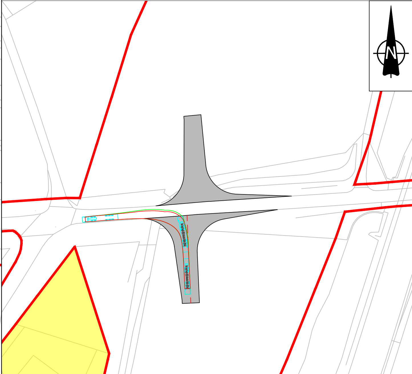
INSET C: 16.5m ARTICULATED VEHICLE TURNING LEFT OUT OF ACCESS ONTO COMMON LANE HEADING WEST - SCALE 1:1000
