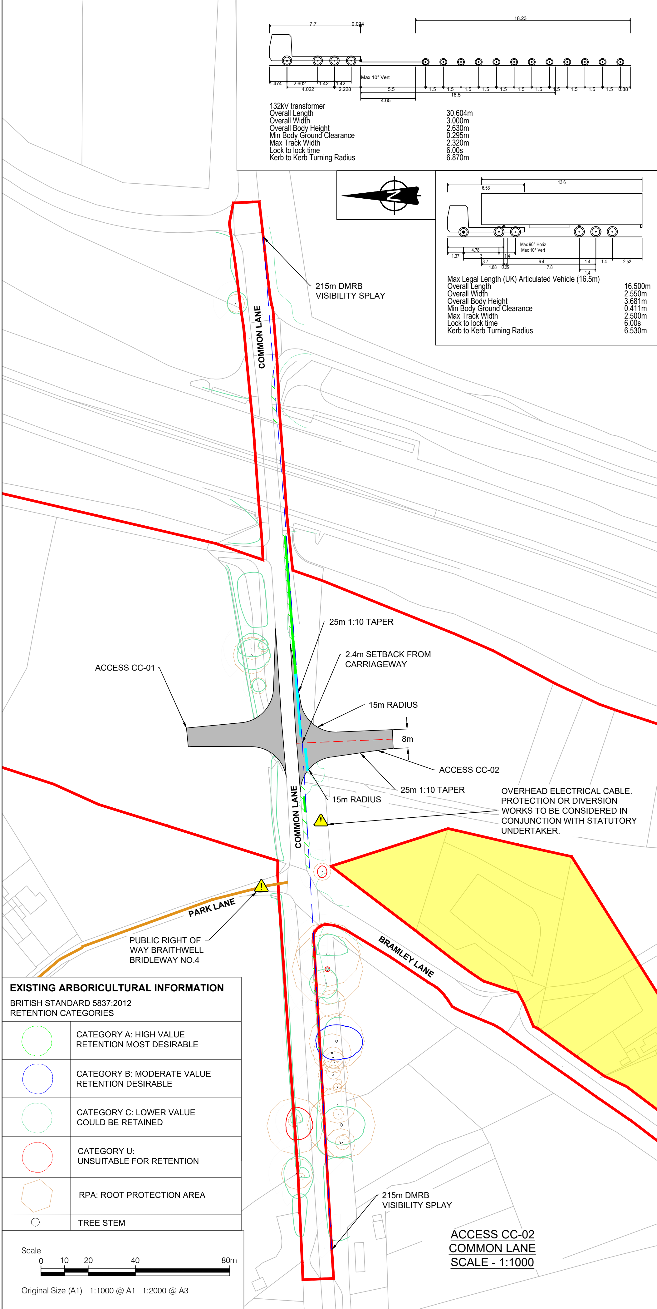
INSET A: 31m 132kV TRANSFORMER VEHICLE TURNING RIGHT OUT OF ACCESS ONTO COMMON LANE HEADING EAST - SCALE 1:1000
