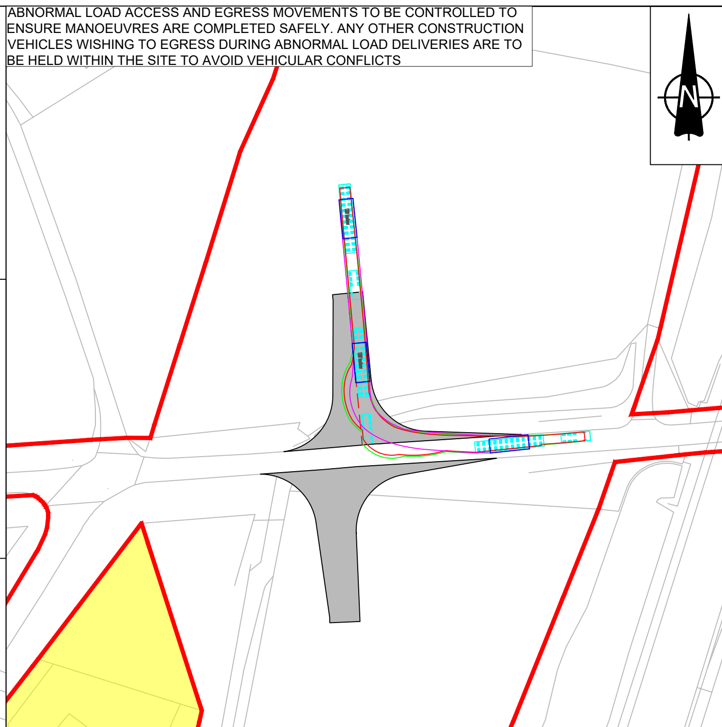
INSET A: 31m 132kV TRANSFORMER VEHICLE TURNING LEFT OUT OF ACCESS ONTO COMMON LANE HEADING EAST - SCALE 1:1000
