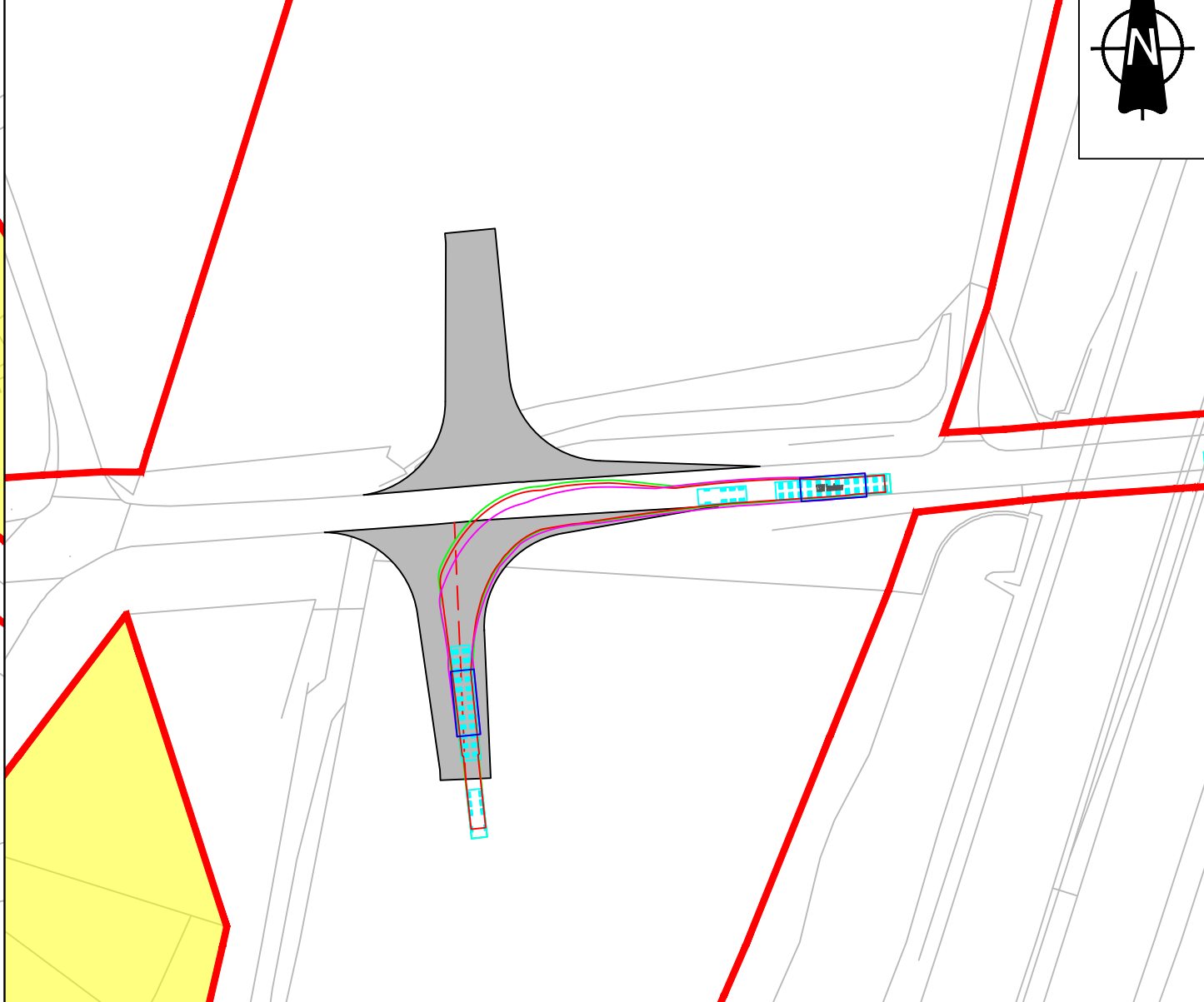
INSET E: 31m 132kV TRANSFORMER VEHICLE HEADING WEST ON COMMON LANE AND TURNING LEFT INTO ACCESS - SCALE 1:1000
