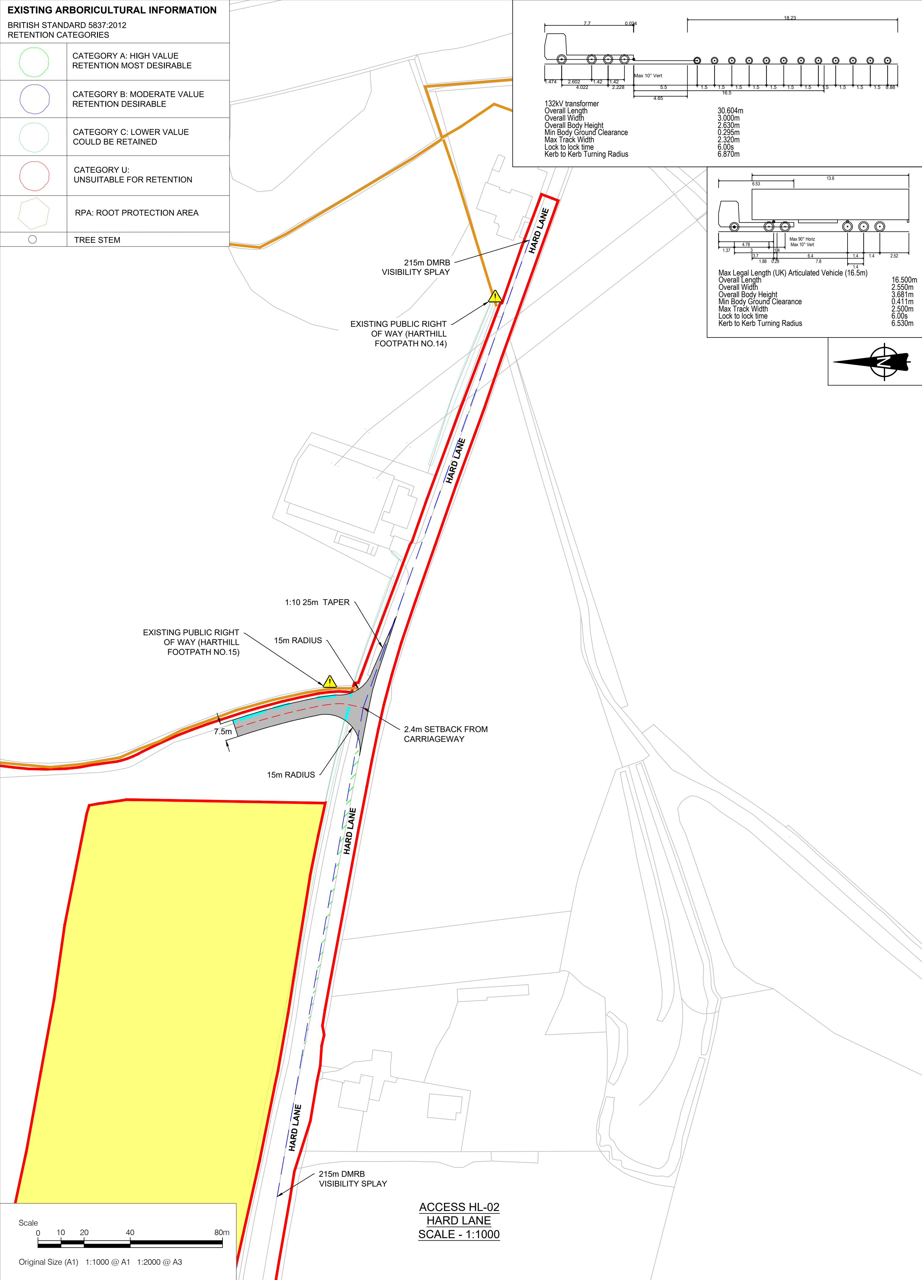
INSET A: 31m 132kV TRANSFORMER VEHICLE SOUTHBOUND RIGHT TURN INTO ACCESS - SCALE 1:1000
