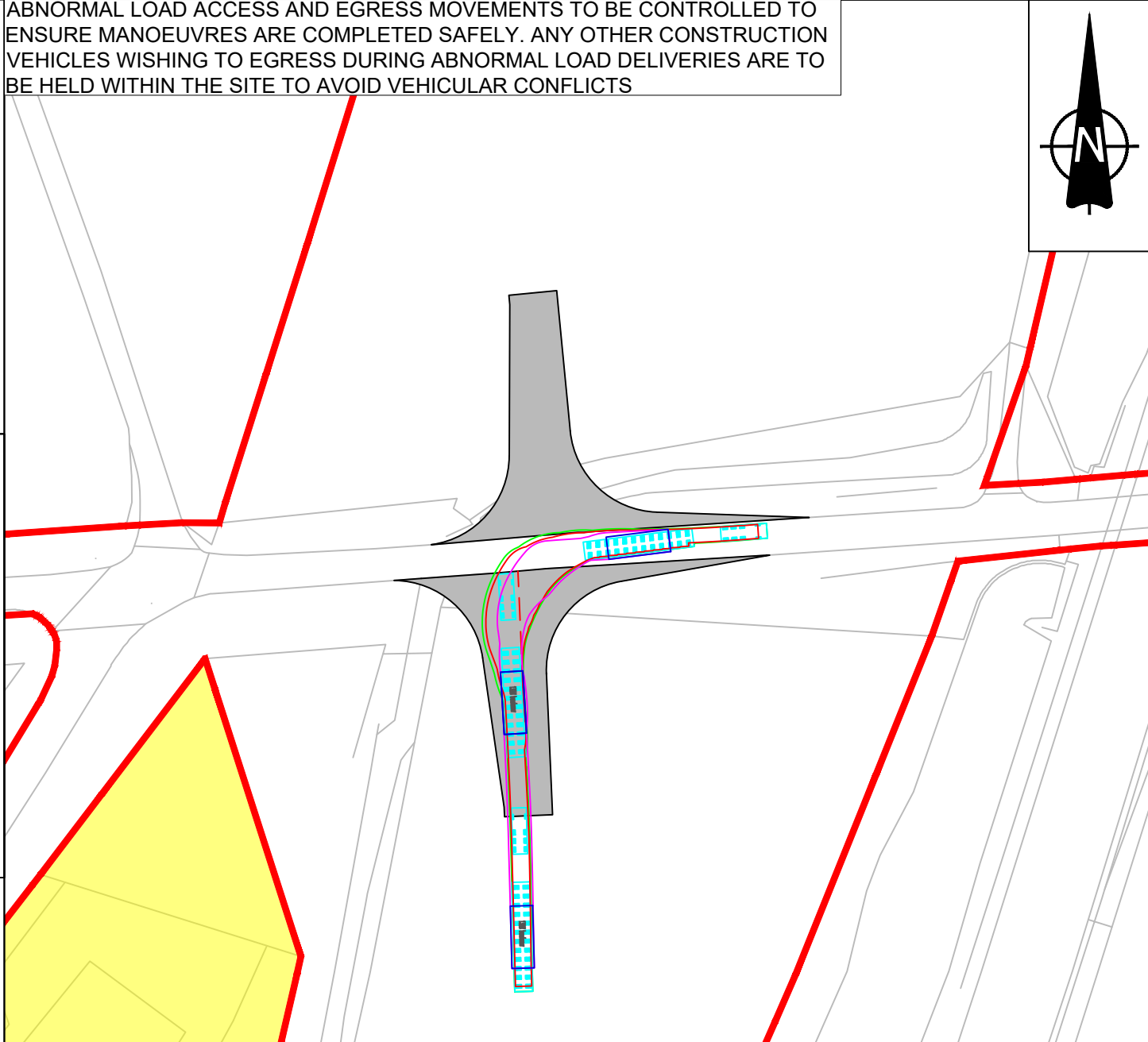
INSET A: 31m 132kV TRANSFORMER VEHICLE TURNING RIGHT OUT OF ACCESS ONTO COMMON LANE HEADING EAST - SCALE 1:1000
